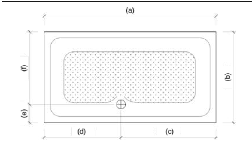
1 Anti-Slip_ShowerTray_Senstec_Rectangular Plan
