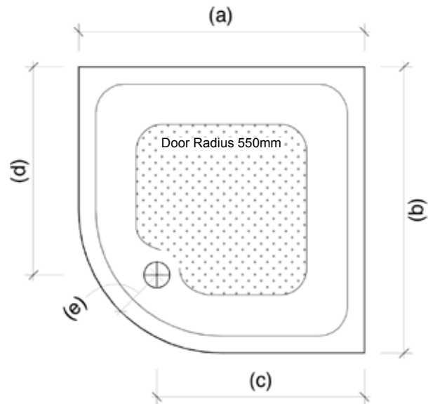
1 Anti-Slip_ShowerTray_Quadrant Plan
