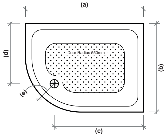
1 Anti-Slip_ShowerTray_Offset Quadrant_LH
